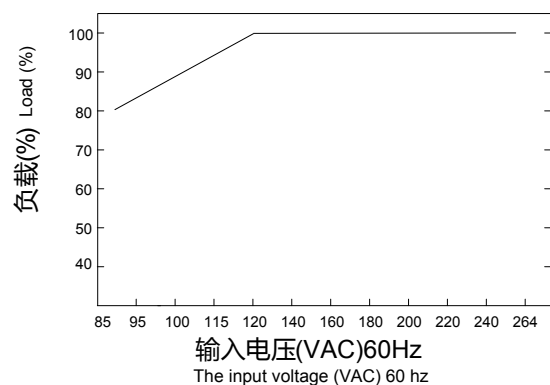
静态特性曲线 The static characteristic curve
