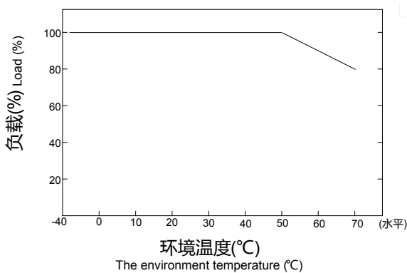
减额曲线 Deduction curve
