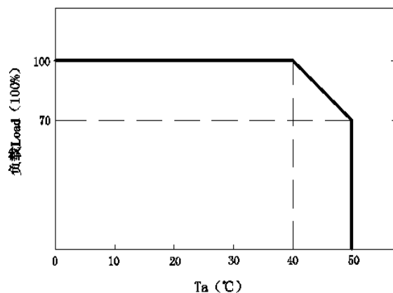
■ 減額曲线Derating Curve
